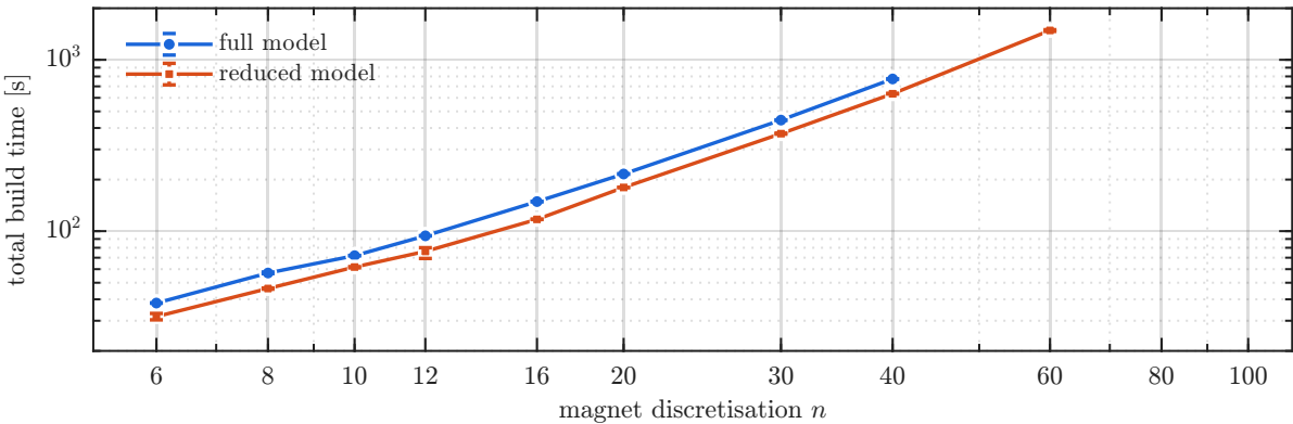
Iteration 2: inline field, -O1 compile
